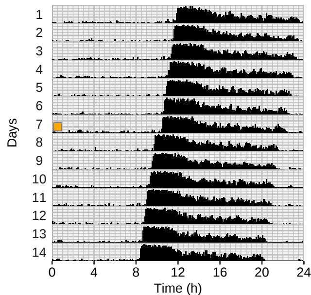
Light pulse at CT = 8
