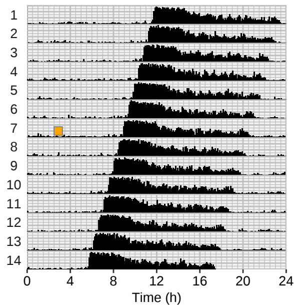
Light pulse at CT = 6
