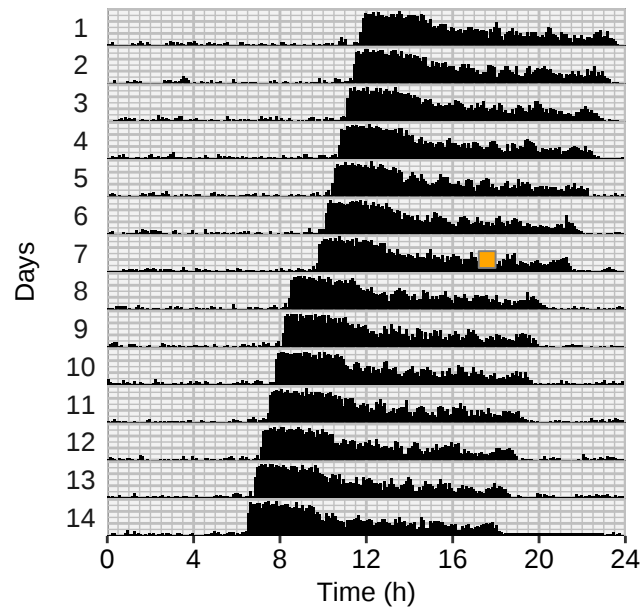
Light pulse at CT = 20
