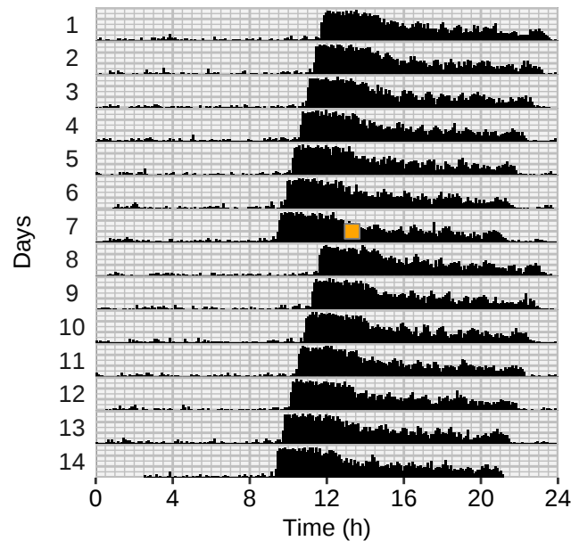
Light pulse at CT = 22
