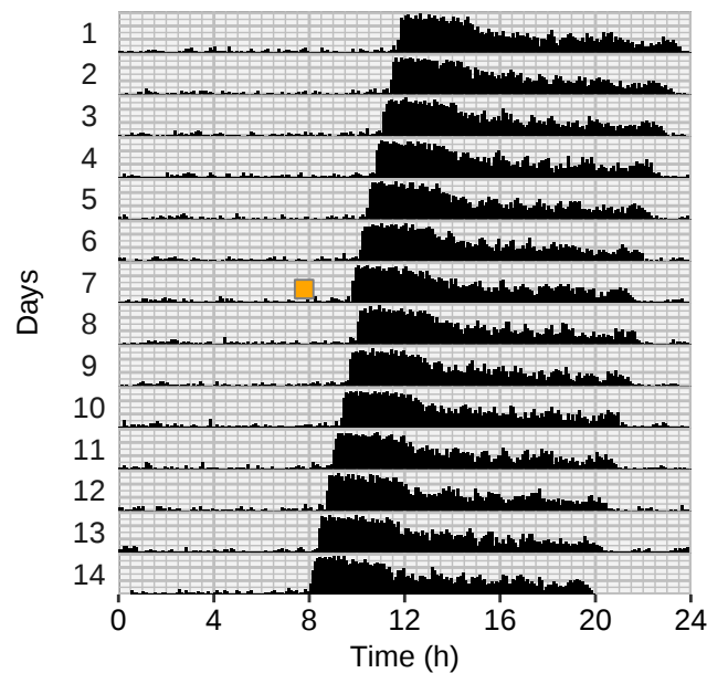
Light pulse at CT = 10
