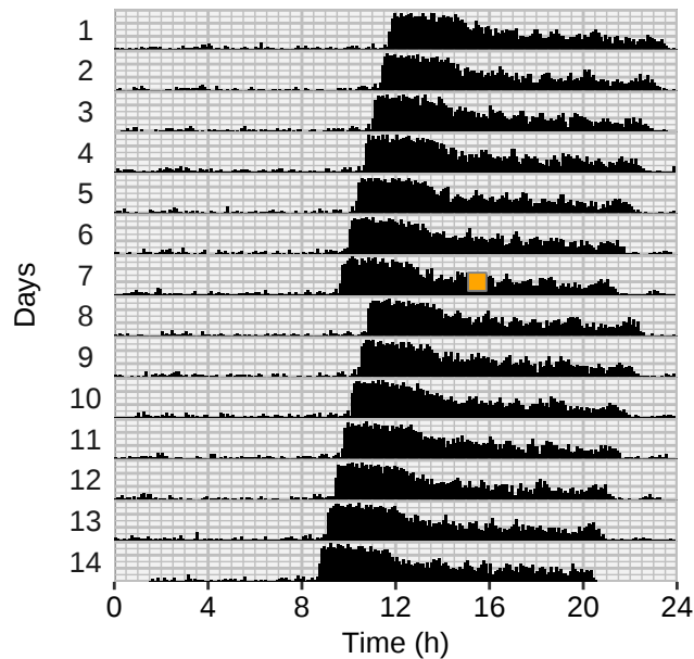
Light pulse at CT = 18
